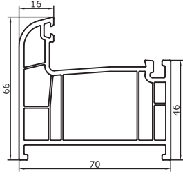
7031 Kasa Profili Frame Profile 1,085 kg/m
